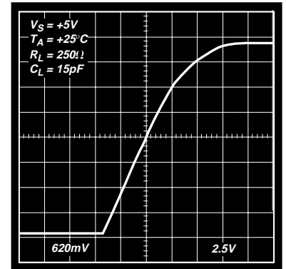
Figure 6. Large Signal Transient Response – Rising
